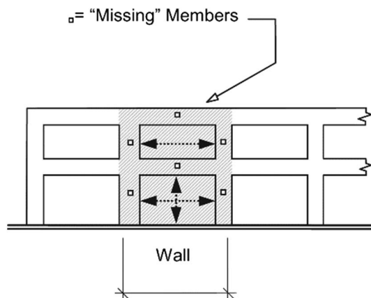
Figure A-15. Incomplete Frame
