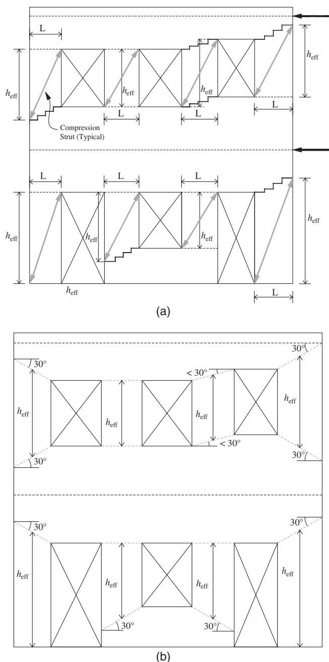
Figure C11-5. URM Rocking Pier Effective Heights. (a) Based on Developing Diagonal Compression Struts That Vary with Direction of Seismic Force; (b) Based on Flexural Cracks Starting at 30^\circ from Opening Corners as per Dolce (1989)
