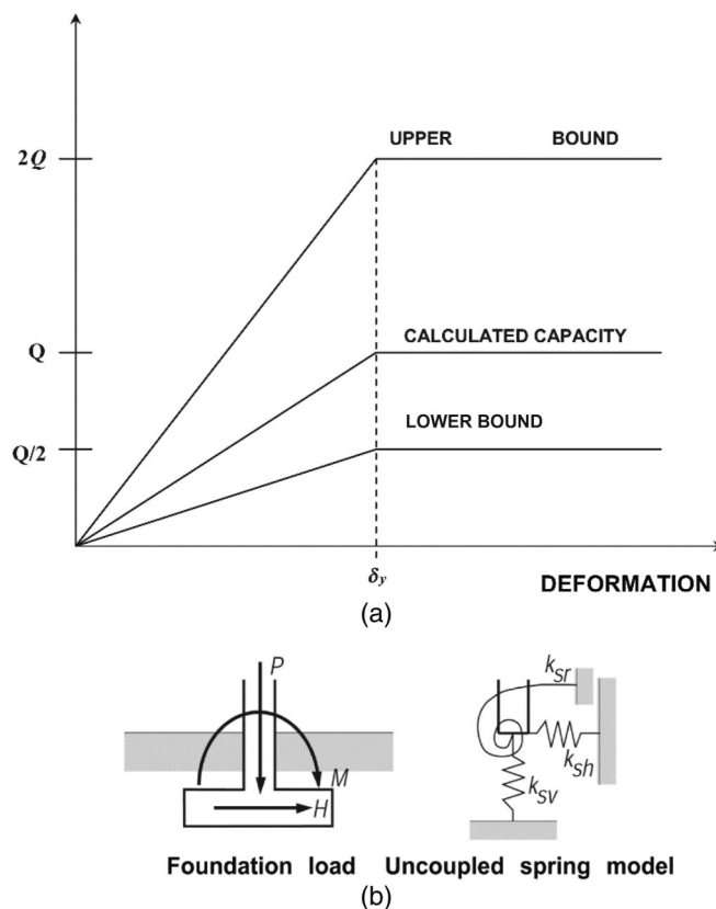
Figure 8-1. (a) Idealized Elastoplastic Load-Deformation Behavior for Soils; (b) Uncoupled Spring Model for Rigid Footings
